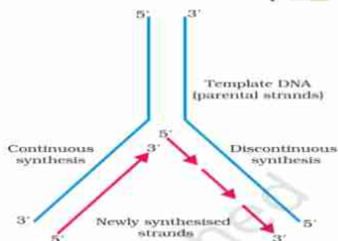
Figure 5.8 Replicating Fork
