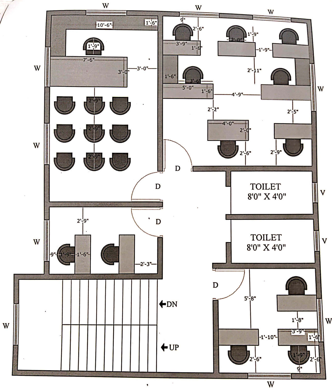
LAYOUT OF FURNITURE ON FIRST FLOOR
