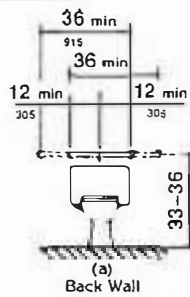
1. Grab bar at wc
