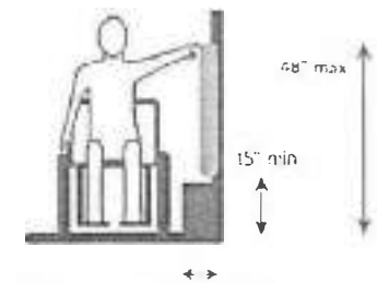
2. Ada compliant reach diagrams
