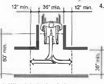
3. Wheelchair circulation
