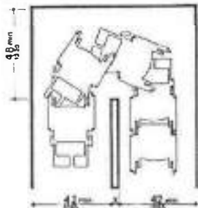
1. Wheelchair circulation
