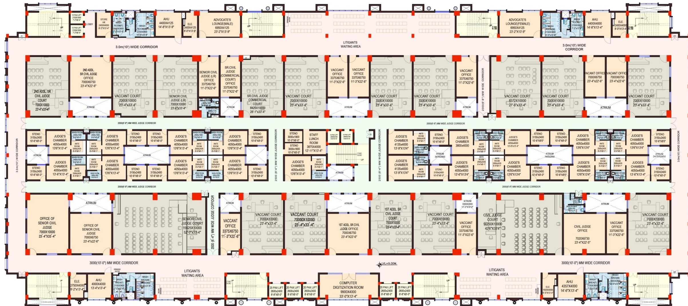
THIRD FLOOR PLAN AREA : 5600 SQ.M.
