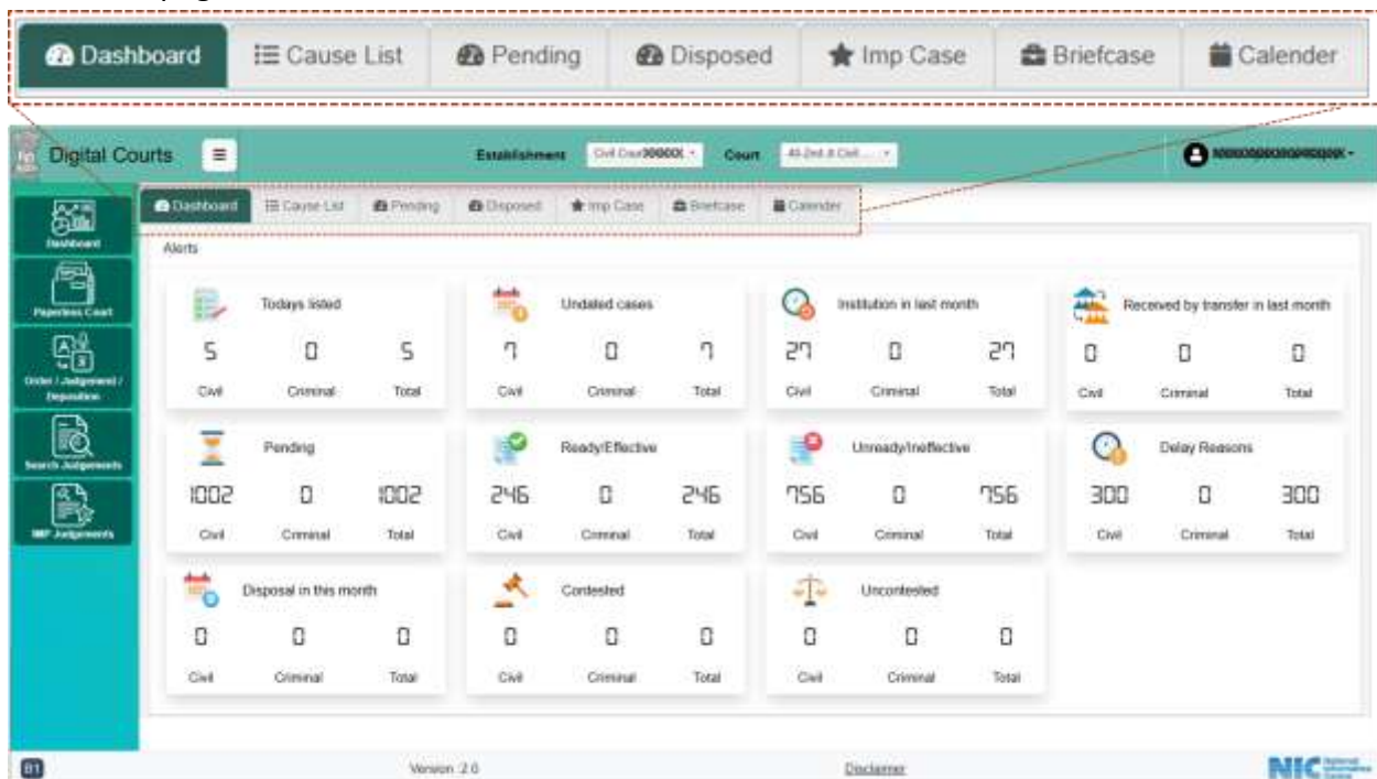
Figure 4: Home Page
