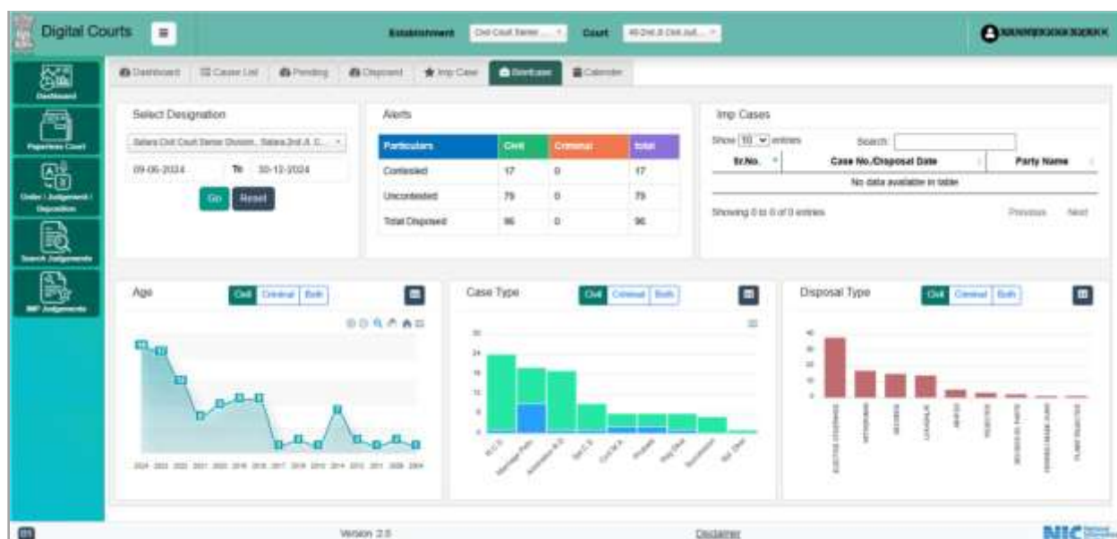
Figure 23: Briefcase
