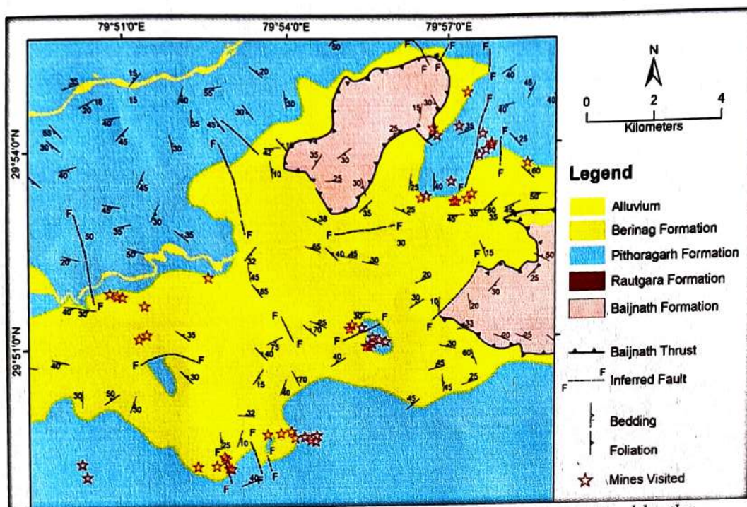
Fig. 2: Geological Map showing the locations of individual mines visited by the committee (Map Source: 1:50K map of GSI).
