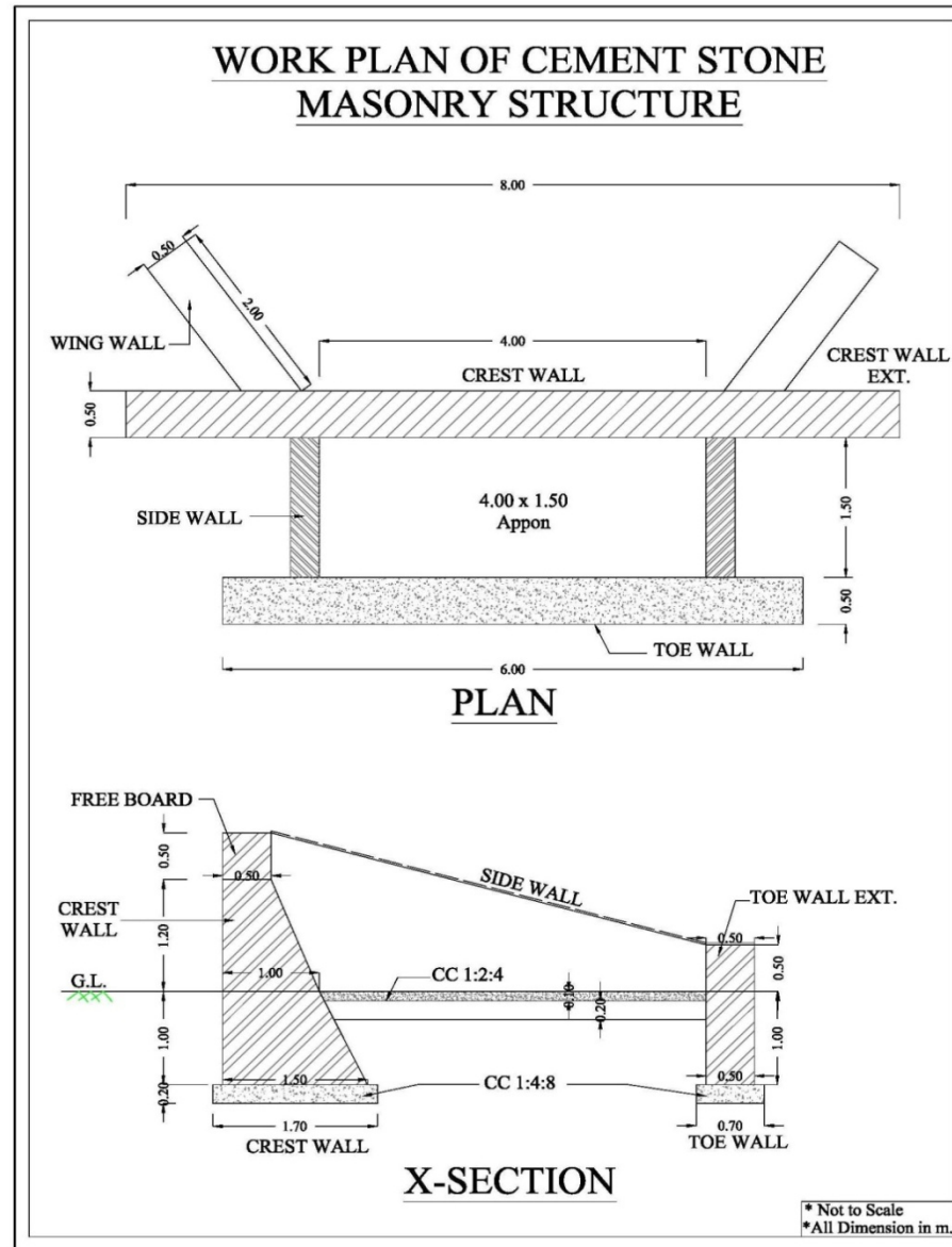
X-section of Masonry Structure
