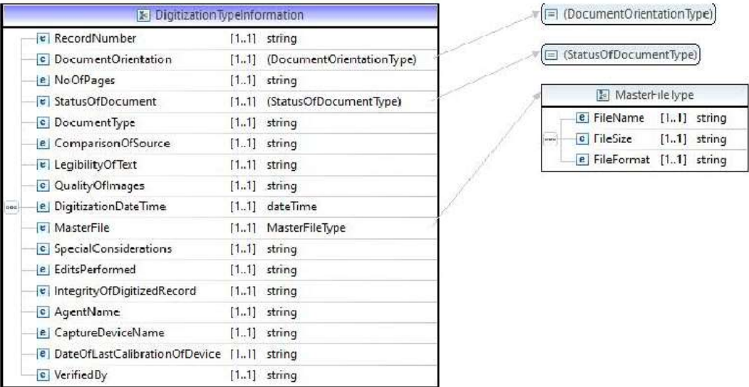
(The XML schema for DVI)
