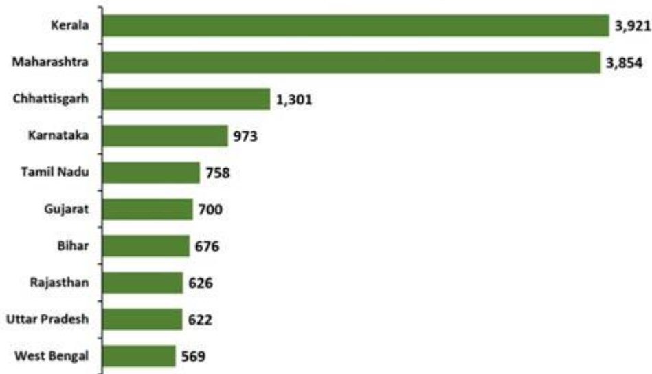
Recovered Cases
