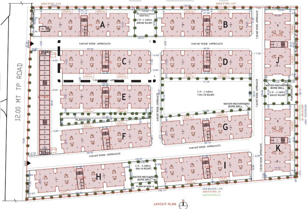
FIGURE 10 Building for compliance check on the layout of project (Example 1)
