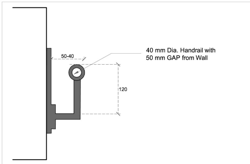
Figure No. 13.14: Fixing Detail of Handrail to the Wall
