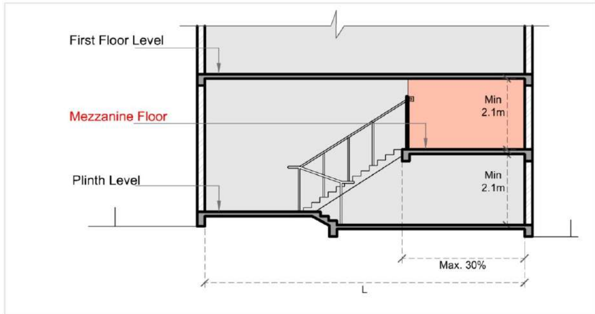
Figure No. 13.12: Mezzanine Floor
