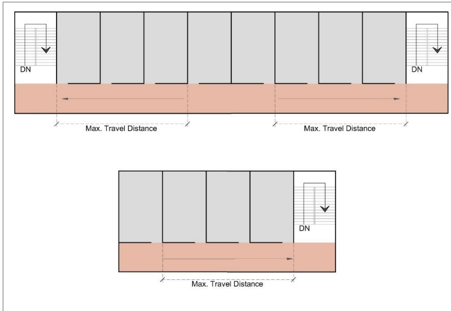
Figure No. 14.3: Maximum Travel Distance to Escape Route
