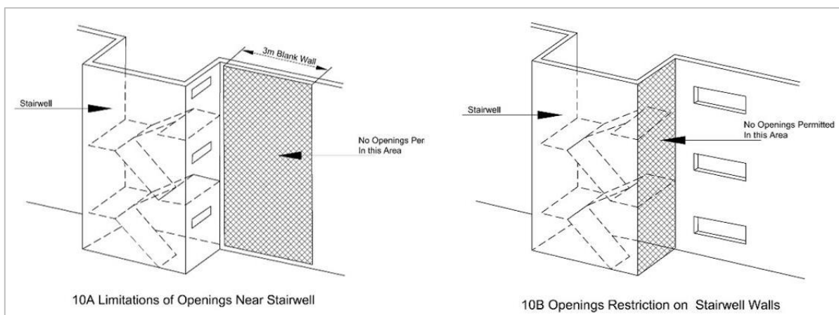
Figure No. 14.11: Opening Restrictions
