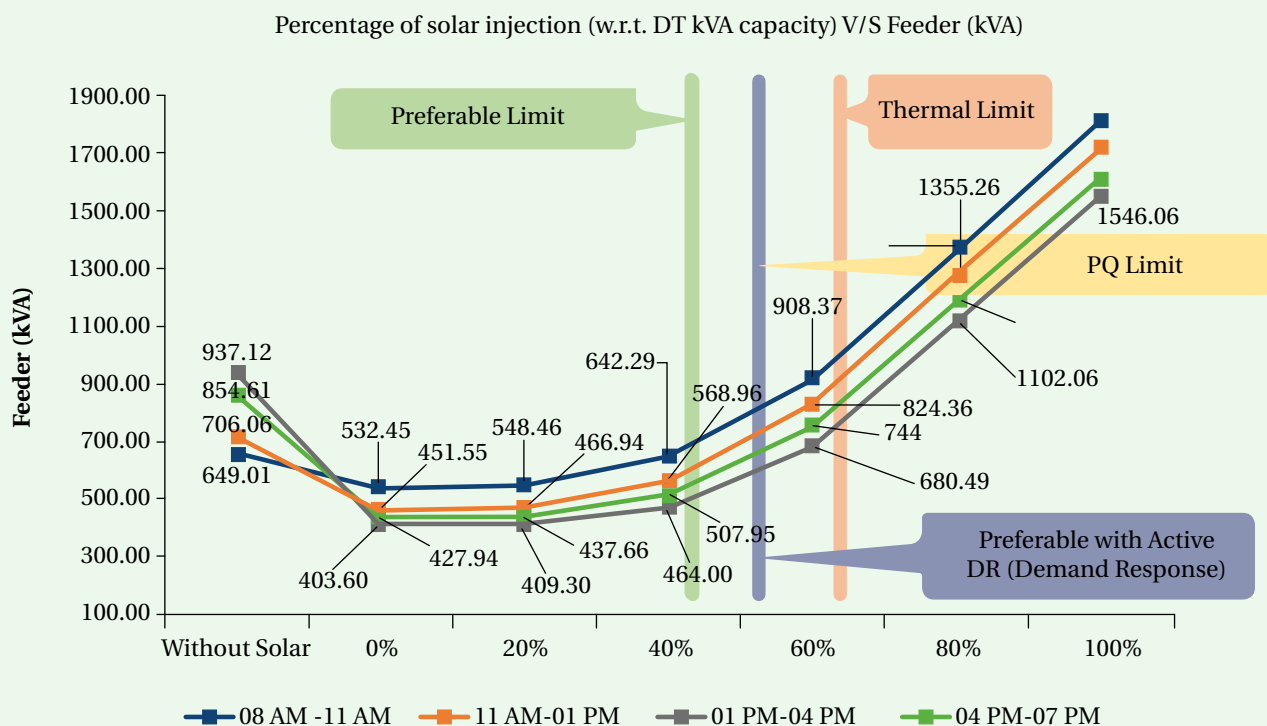
Figure 18: UHBVN Feeder Load Flow Analysis
