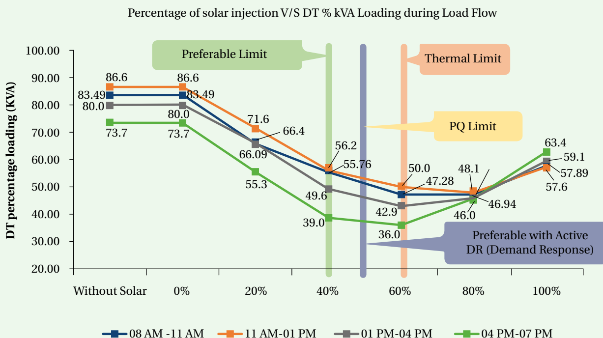
Figure 21: CESC Feeder Load Flow Analysis
