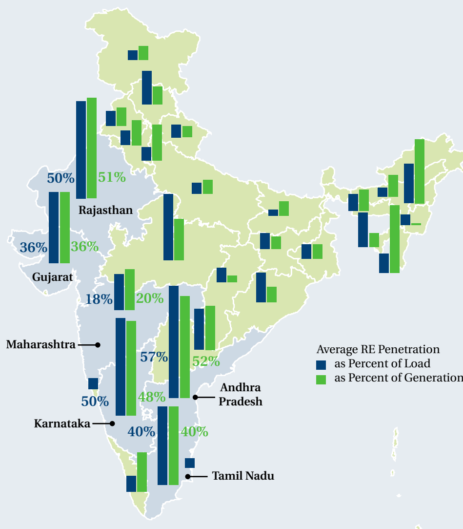
Figure 52: RE penetration as percentage of Generation and Load
