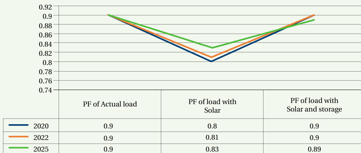
Figure 31: Increment of PF by Using Storage
