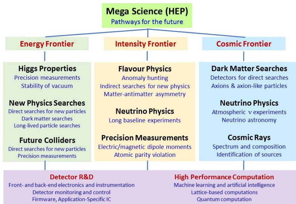
Figure 1.3 Summarising some of the important scientific goals of the High Energy Physics community.
