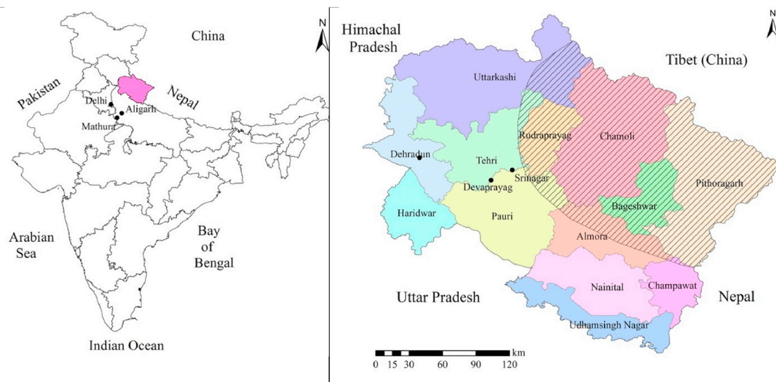
Fig. 1. Location map of the study area; Uttarakhand in India (left). Hatched area in the map of the province (right) represents Zone V of Earthquake Zoning Map of India while unhatched area represents Zone IV.
