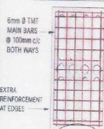
REINFORCEMENT DETAIL (TYP.)
