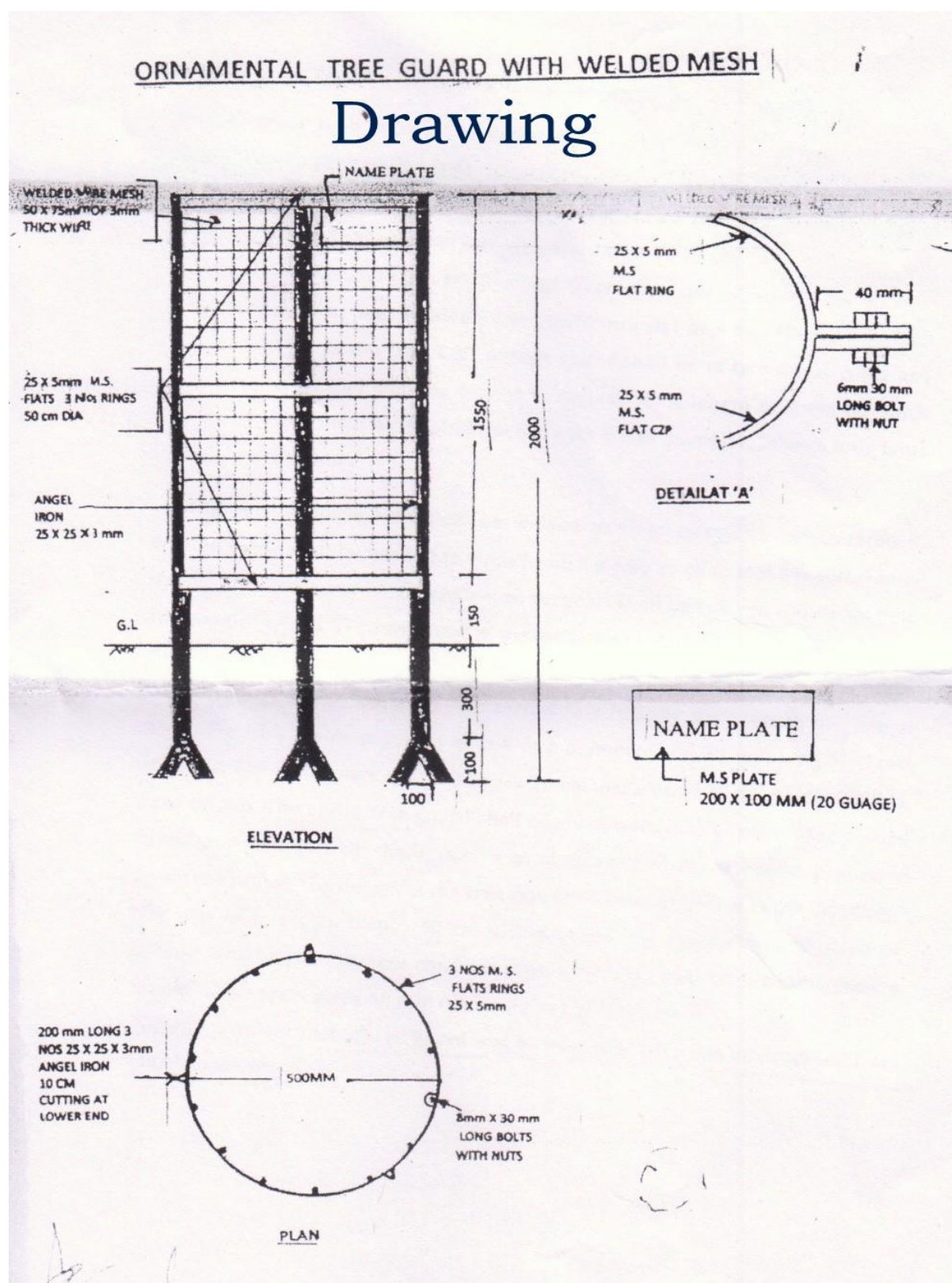
Annexure-II (Drawing of Tree Guard) Fig. 1
